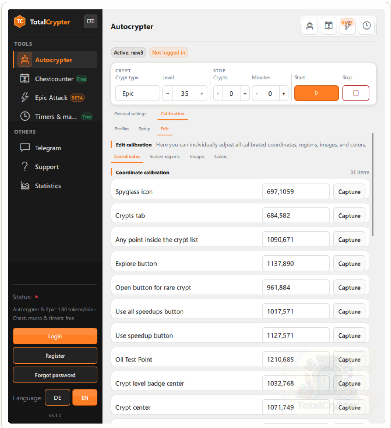
Edit calibration
