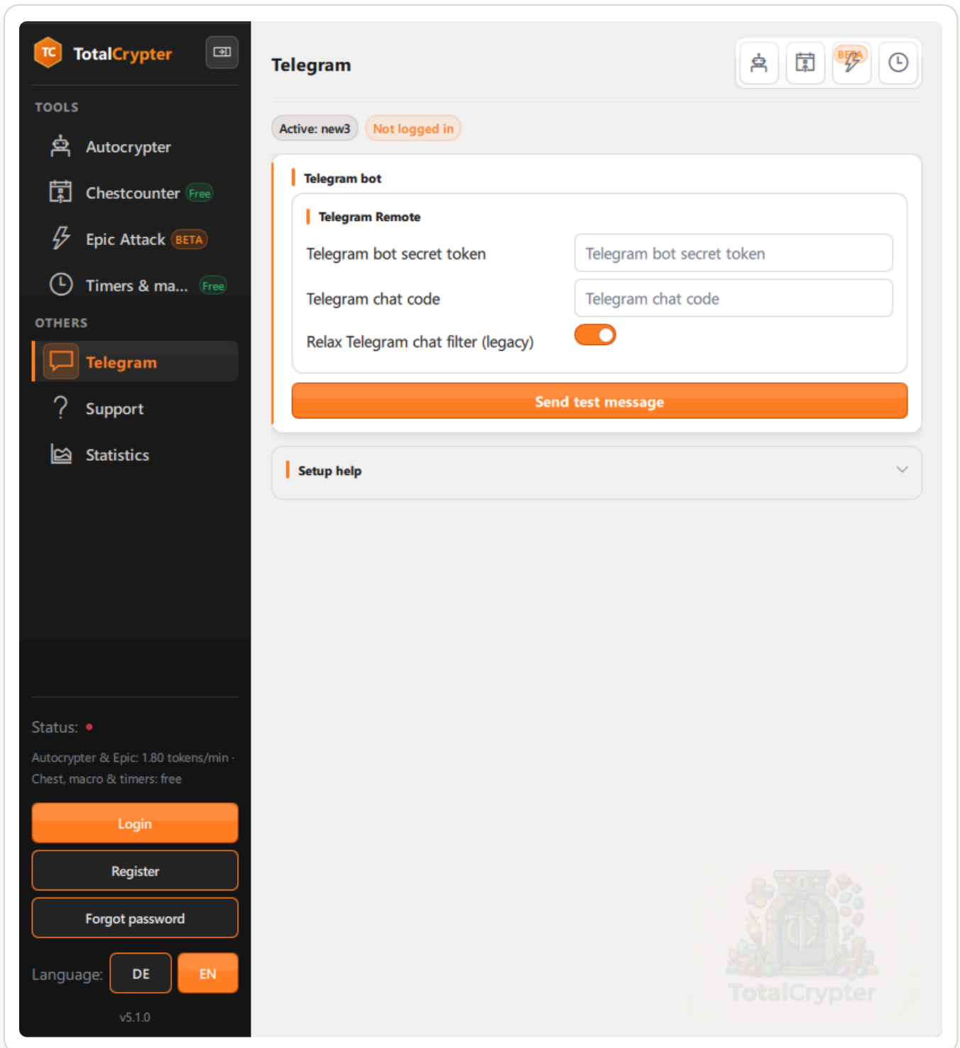
Telegram settings
